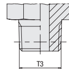
Taper Thread Metric Taper Thread DIN 3852-1 (Form C) Whitworth Taper Pipe Thread DIN 3852-2 (Form C)
