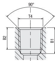
Port (Taper Thread) for Male Studs with National Pipe NPT Thread ANSI/ASME B1.20.1-1983
