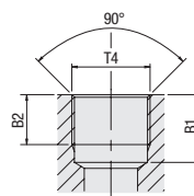
Port (Parallel Thread) for Male Studs with Metric Taper Thread DIN 3852-1 (Form Z) for Male Studs with Whitworth Taper Pipe Thread DIN 3852-2 (Form Z)
