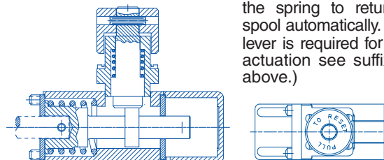
Suffix Detail-3358AE
