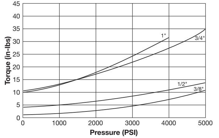
Torque vs. Pressure
