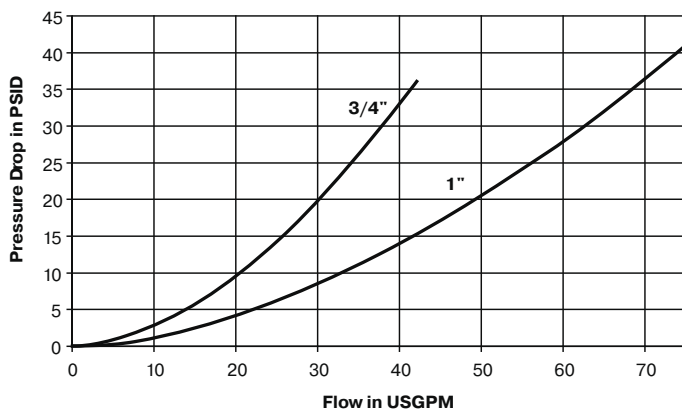
60 Series (3/4" & 1") Test Fluid: Oil - 150 SUS
