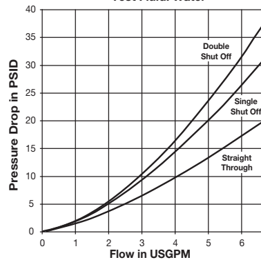
Performance Spectrum Series (3/8") Test Fluid: Water
